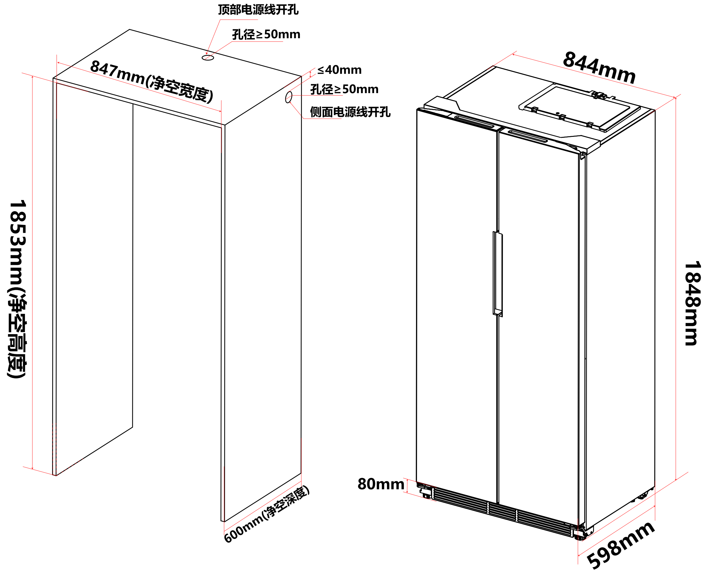
Traditional Side by Side (平嵌对开)
