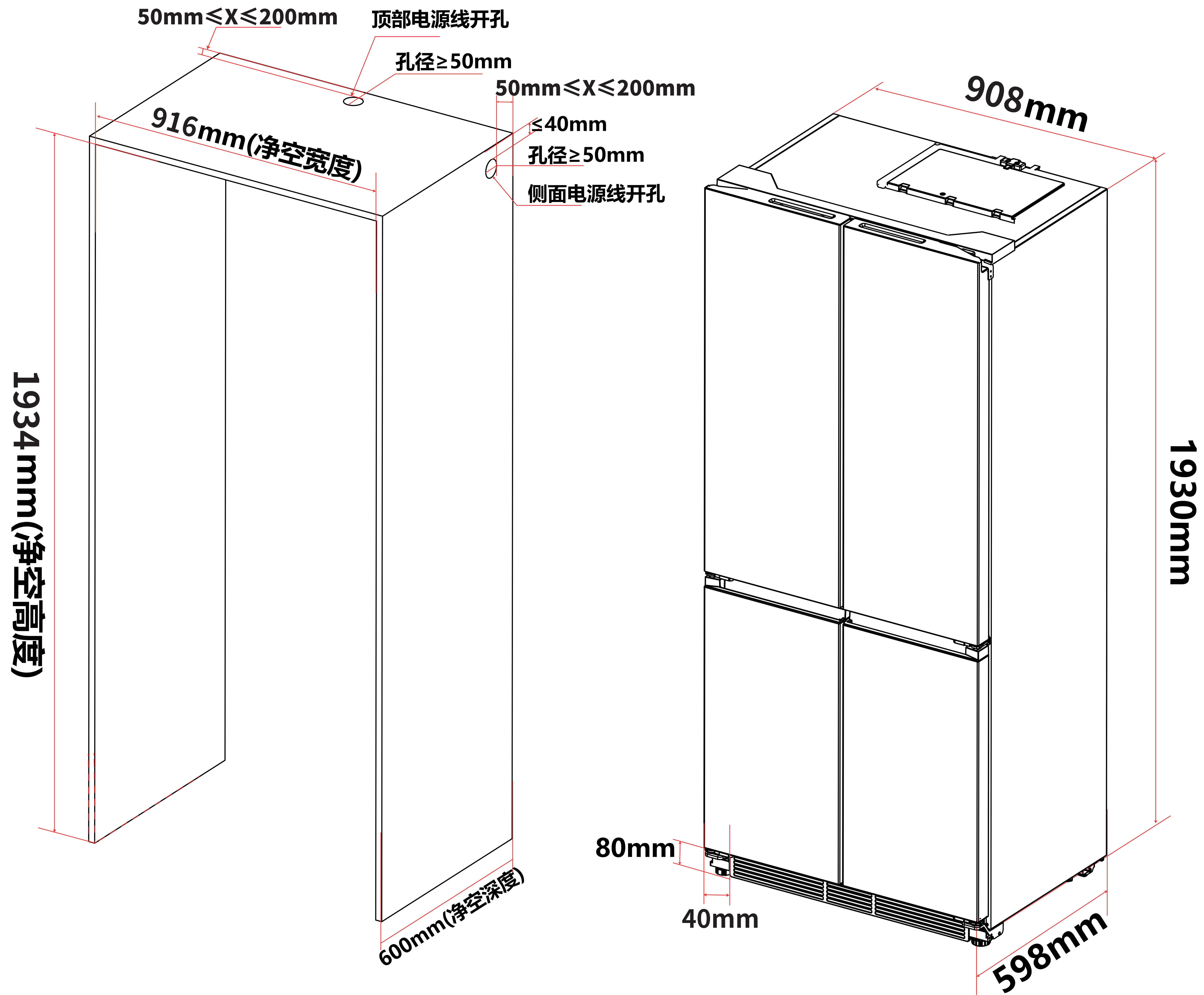
Traditional Cross Door (平嵌十字)
