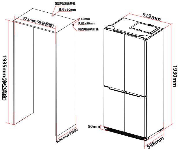
Traditional Cross Door (平嵌十字)
